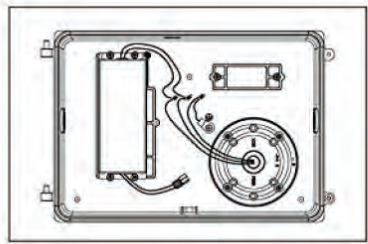
loosen screws and remove the front part
