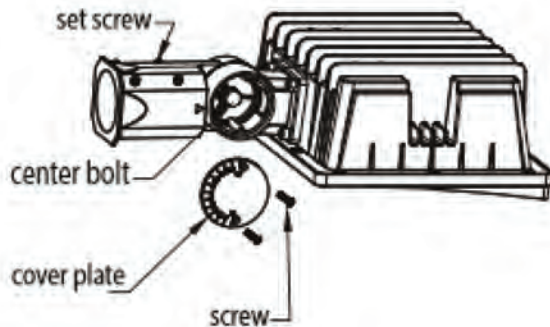
Slipfitter Mounting
